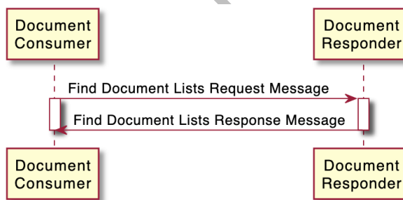
Figure 7 Interaction diagram for [ITI-66]
